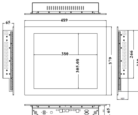
PMPPC-1908-(Skylake/KabyLake CPU) Drawing
