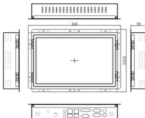
OFPPC-1216-J1900 Drawing
