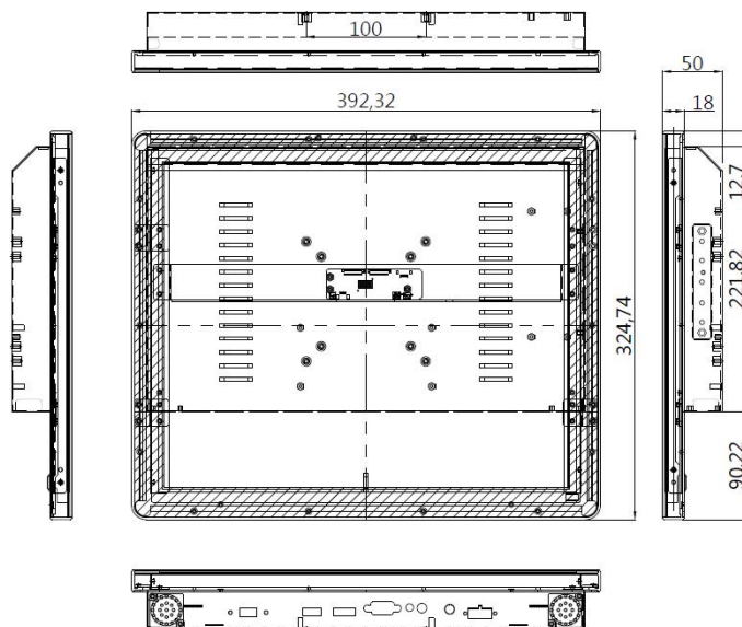
TM1700P-Drawing
